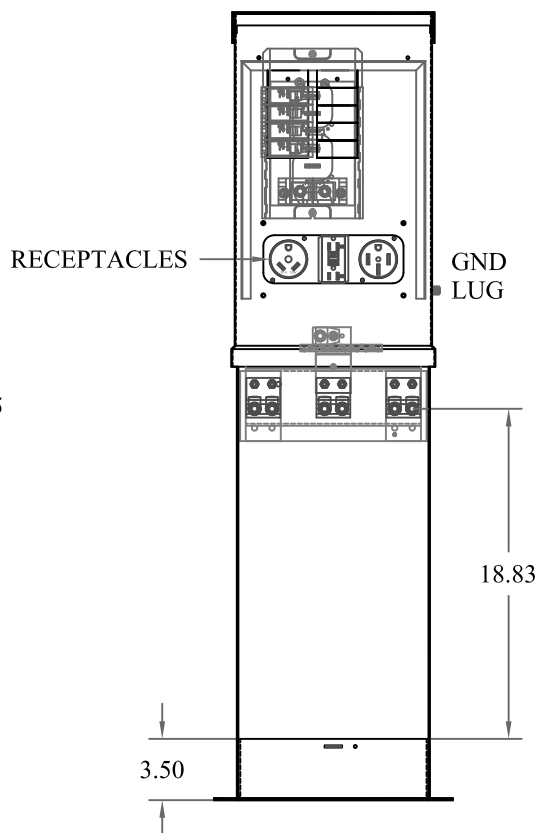
FRONT VIEW SHOWN LESS COVERS
