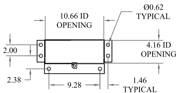
FRONT VIEW SHOWN LESS COVERS
